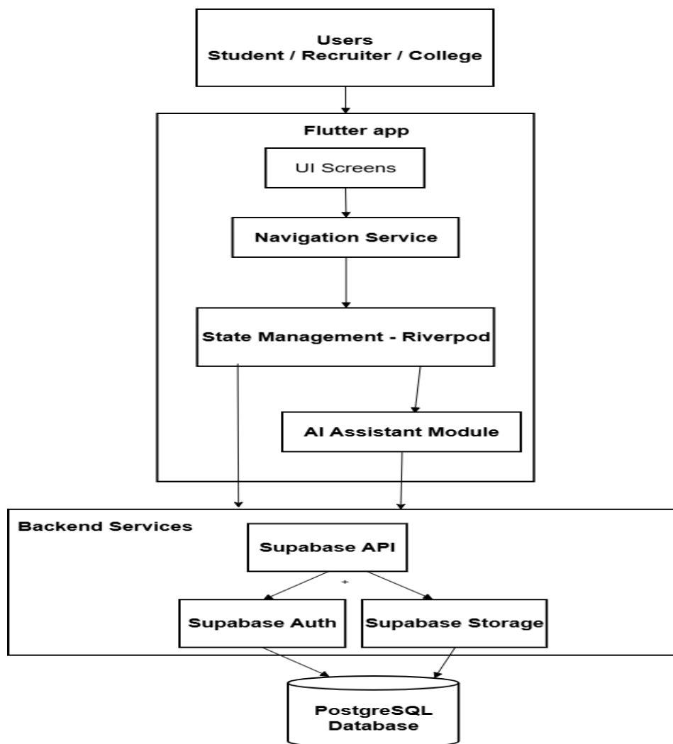
Figure 3.2.1: High-Level Architecture
